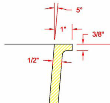
Flange Detail
