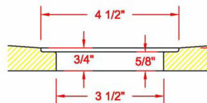
Drain Detail
